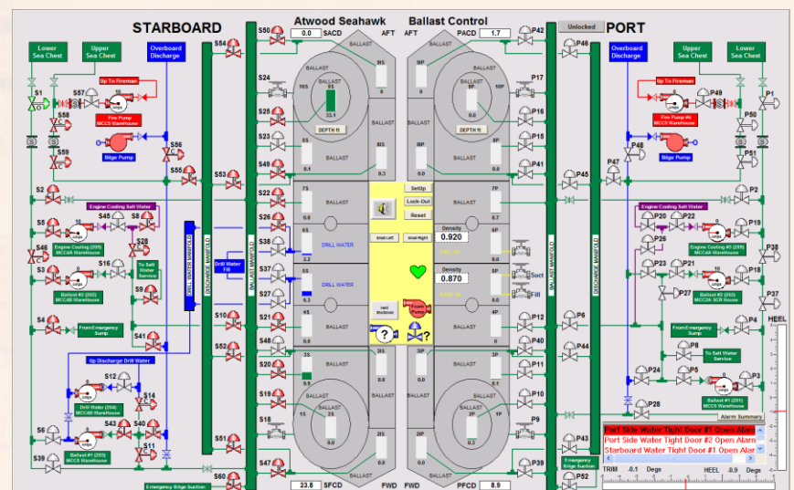
Ballast Control / Monitoring System
